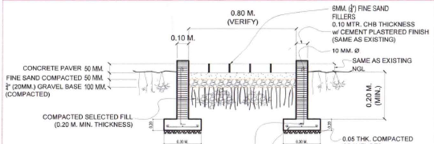
TYPICAL CONCRETE PAVER w/ 100MM. THK. CHB EDGING & RETAINER DETAILED
