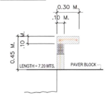
DETAILED SECTION OF CHB WALL NOT TO SCALE
