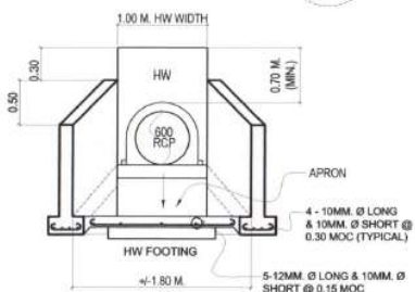
SECTION/ELEVATION B-B
