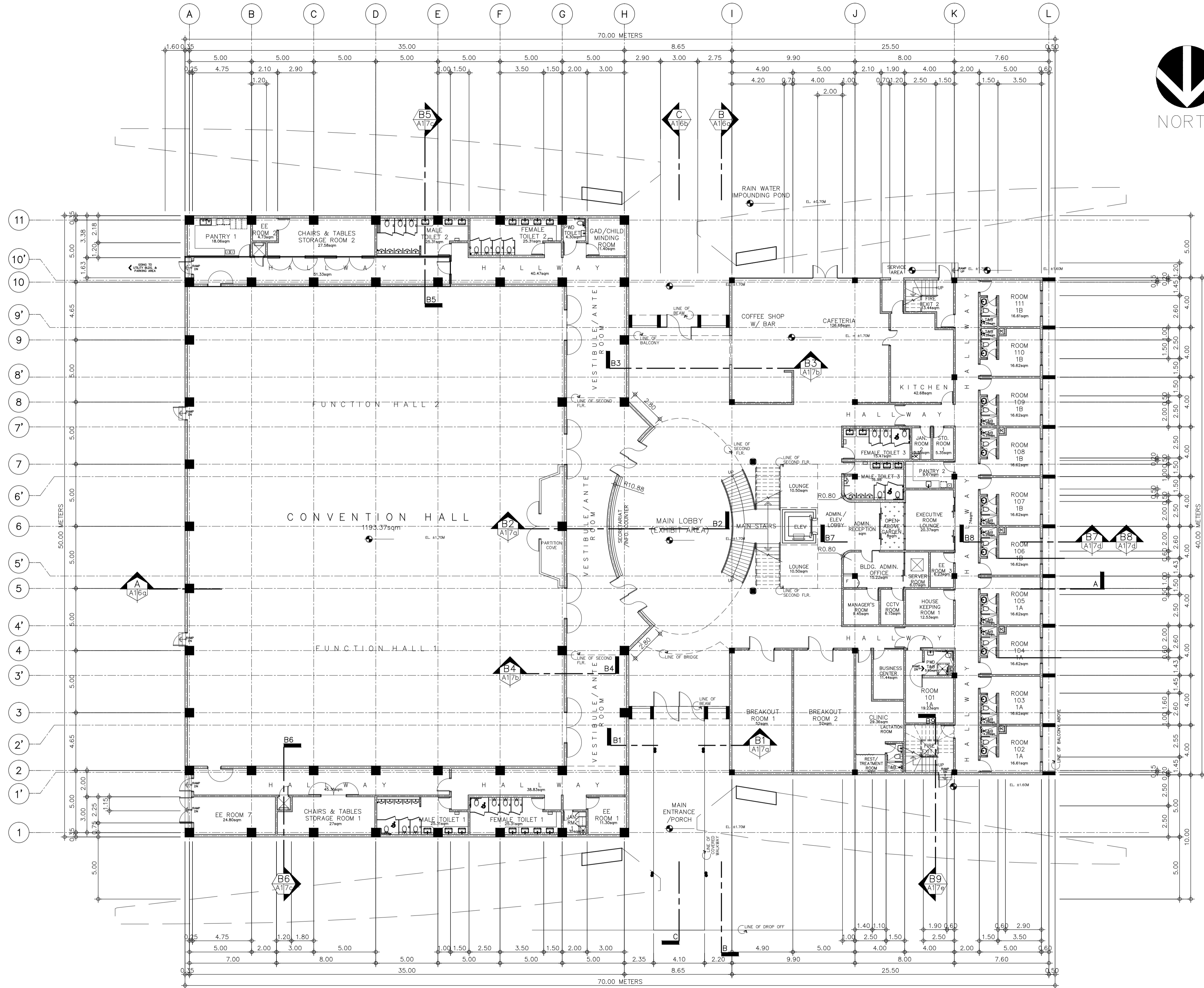
A GROUND FLOOR PLAN A1 1 SCALE 1:175M
