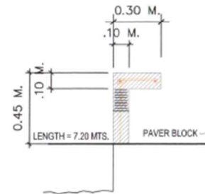
DETAILED SECTION OF CHB WALL NOT TO SCALE
