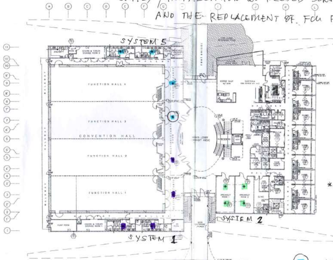
GROUND FLOOR MECHANICAL LAYOUT SCALE 1:1750
