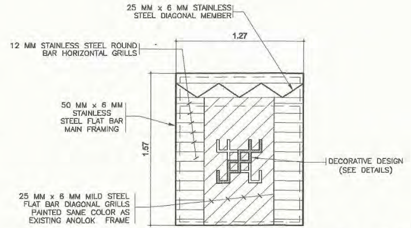
E) AT WINDOW 2 (4 SETS @ 1st FLOOR, 5 SETS @ 2nd FLOOR) SCALE 1:25 M.
