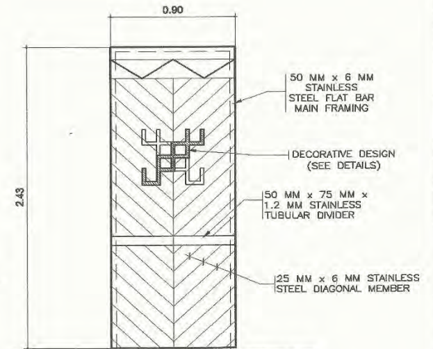
J) AT DOOR 2 (1 SET @ 1st FLOOR) SCALE 1:25 M.
