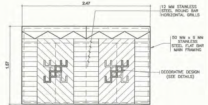
D) AT WINDOW 1 (4 SETS @ 1st FLOOR) SCALE 1:25 M.
