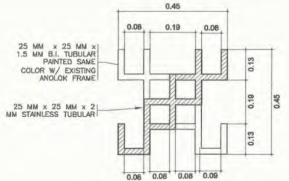
DECORATIVE DESIGN DETAIL FOR OTHER AREAS SCALE 1:10 M.
