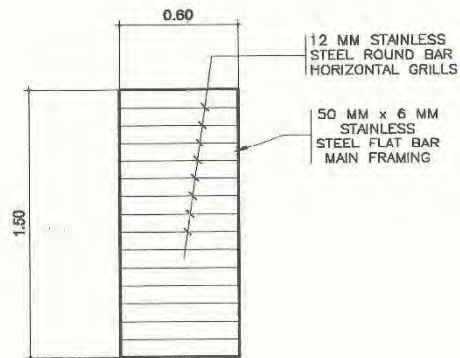
F) AT WINDOW 3 (1 SET @ 2nd FLOOR) SCALE 1:25 M. (INTERIOR MOUNTED)
