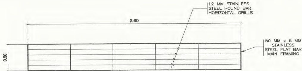
G) AT WINDOW 4 (1 SET @ 1st FLOOR) SCALE 1:25 M. (INTERIOR MOUNTED)
