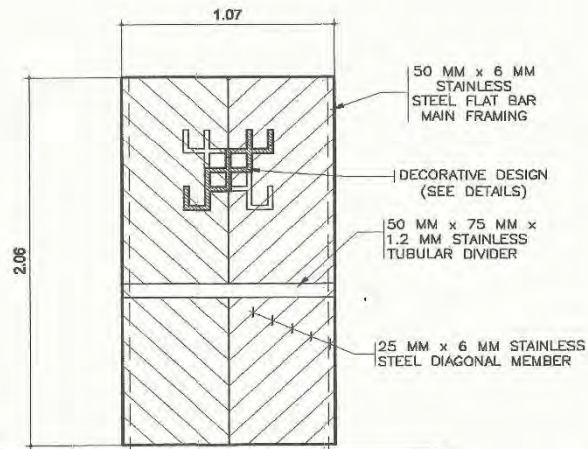
I) AT DOOR 1 (2 SETS @ 1st FLOOR) SCALE 1:25 M.
