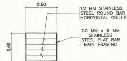
H) AT WINDOW 5 (12 SETS @ 1st FLOOR, 19 SETS @ 2nd FLOOR) SCALE 1:25 M. (INTERIOR MOUNTED)
