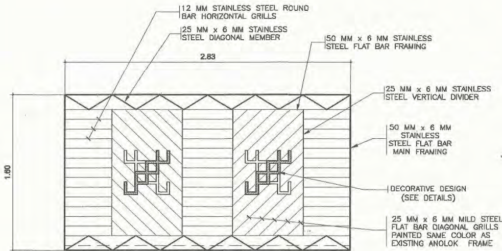
C) AT BALCONY (12 SETS @ 1st FLOOR, 19 SETS @ 2nd FLOOR) SCALE 1:25 M.
